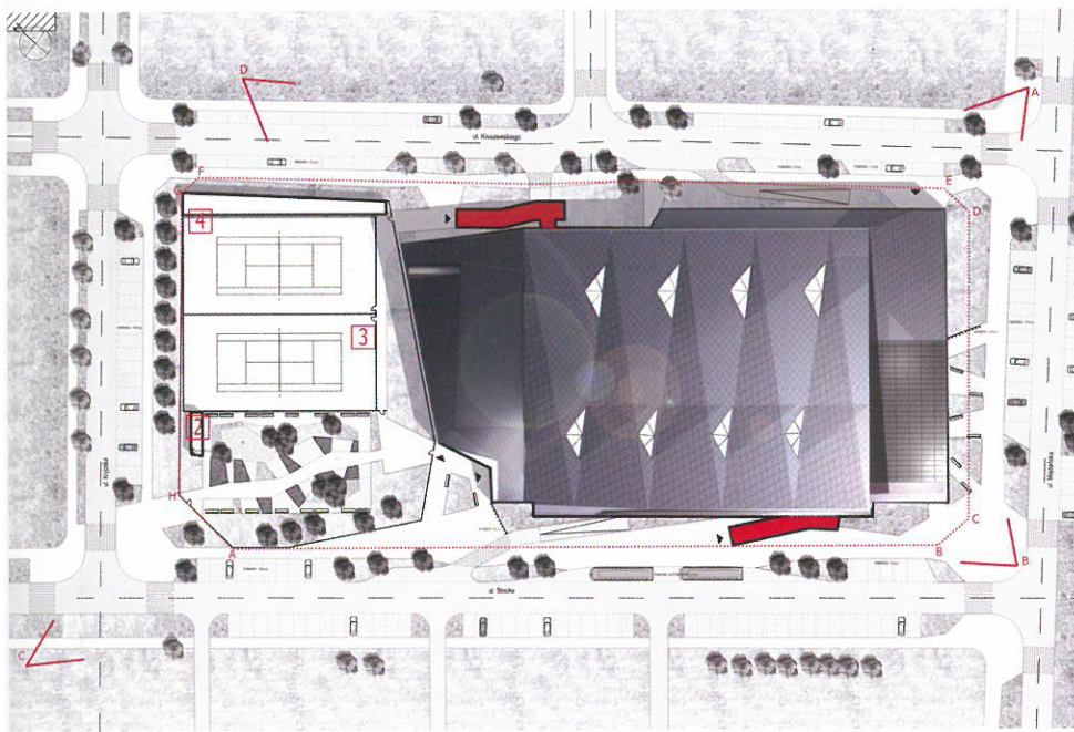
Site Plan
