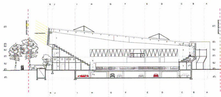
Section B-B'
